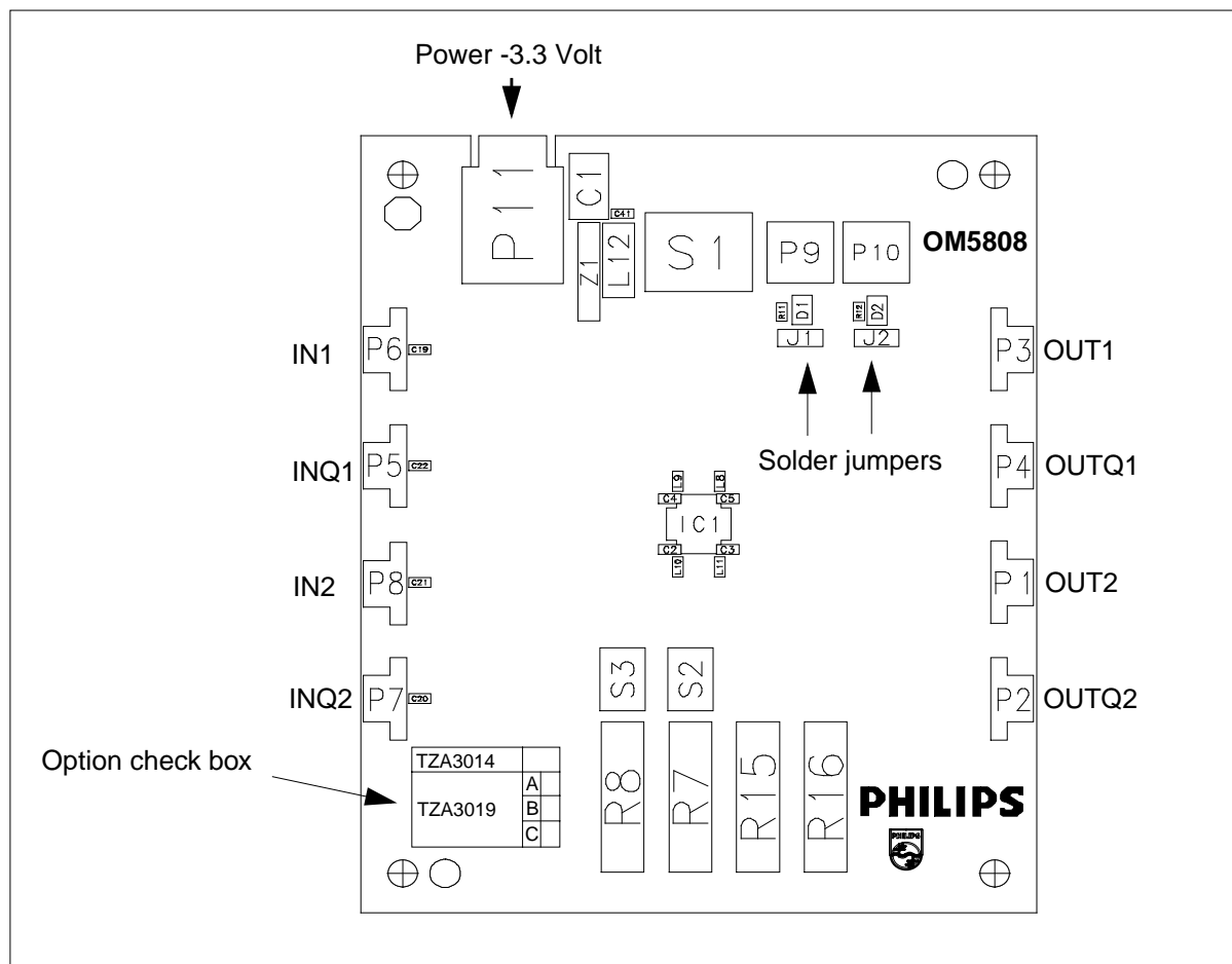
Fig.2 OM5808 demo board
